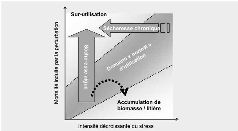
FIGURE 3 : Effects of drought spells in pastures according to intensity and frequency. The mortality effect (disturbance) and the effect of fall in production (stress) may trigger off mechanisms in the vegetation dynamics and require also a re-adjustment of the management practices (the basic model is that of figure 1b).
