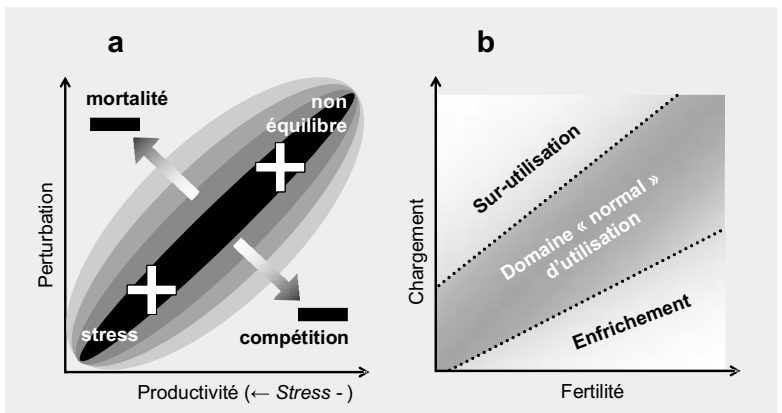
FIGURE 1 : Processes responsible for the maintenance of the plant diversity in grassland communities : a) high (+) or low (-) levels of diversity depend on particular combinations between two types of constraints (stresses and disturbances, theoretical model) ; b) practices of grassland management seen from the points of view of two types of constraints (fertility and stocking rate), the combinations of which determine the rate of utilization of the plant production (empirical model, after BALENT, 1991 and BALENT et al. , 1998, 1999).
